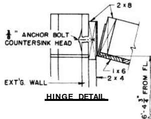
DETAIL SECTIONS
