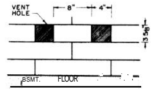
AIR VENT DETAIL
