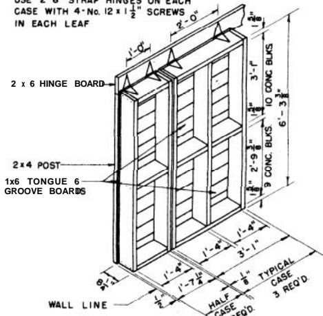
ISOMETRIC OF CASES
